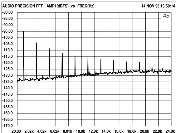
16 bit input signal -100 dB high pass dither applied
