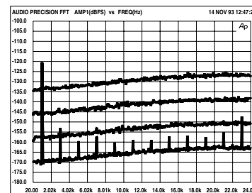
Fig. 6 - dither only 16 (top), 18, 20, and 22 bits -120 dB 1 kHz sine tone
