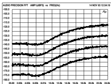
Fig. 4 - \alpha coustic \beta it Correction™ 16 (top), 18, 20, and 22 bit no input signal
