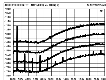
Fig. 5 - ABC HP-NS2 16 (top), 18, 20, and 22 bit -120 dB 1 kHz sine tone
